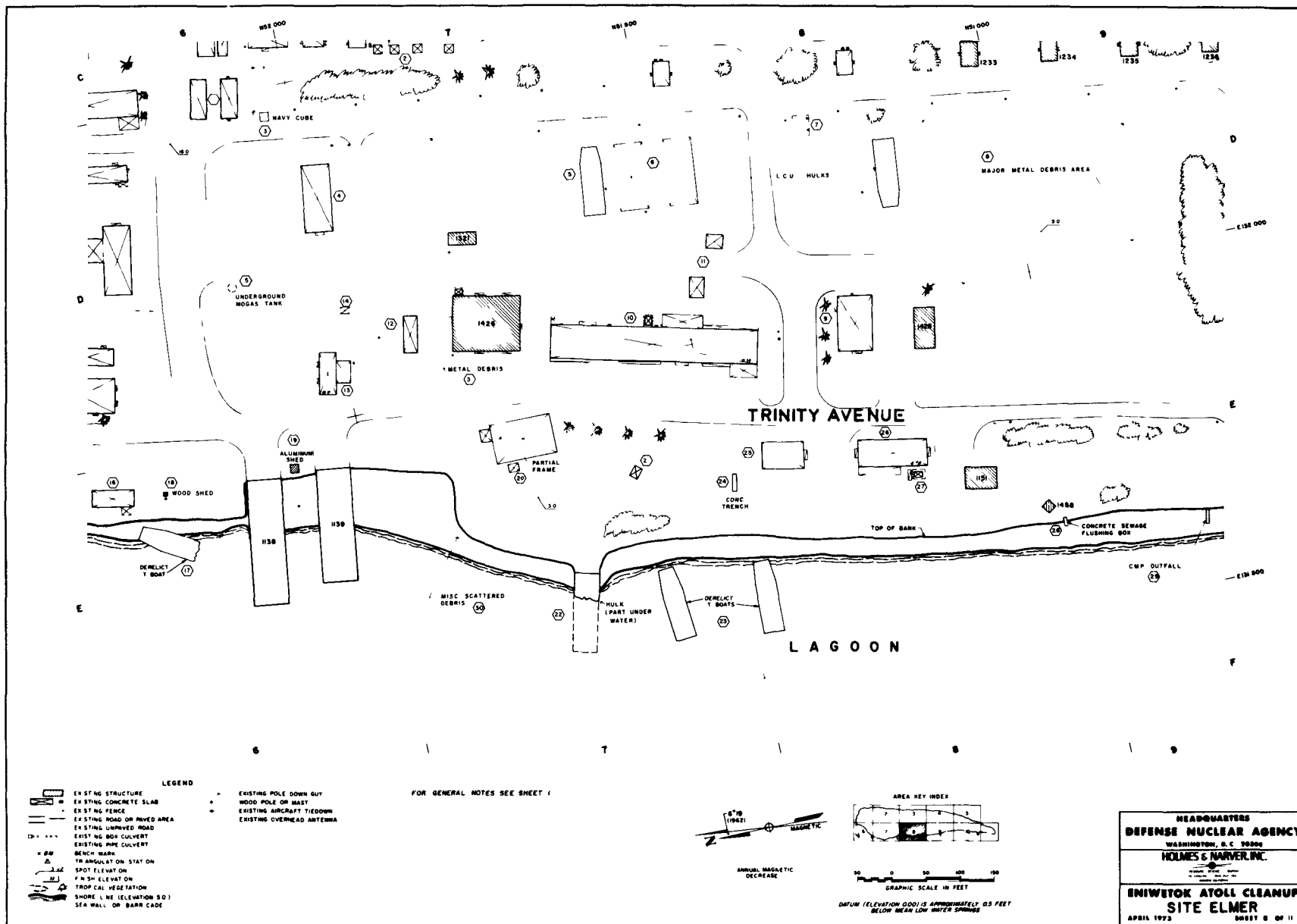
FIGURE 149. SITE ELMER, SHEET 8 OF 11
